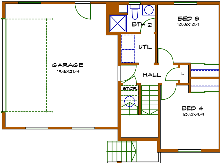
ALT. LOWER FLOOR PLAN AREA THIS FLOOR: 466 SF
