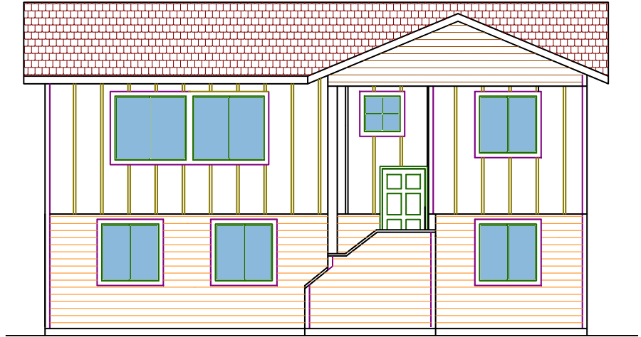
ALT. FRONT ELEVATION
