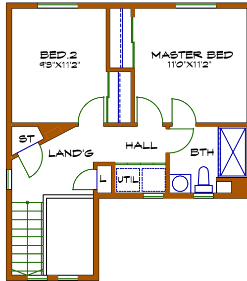
UPPER FLOOR PLAN AREA: 456 SF
