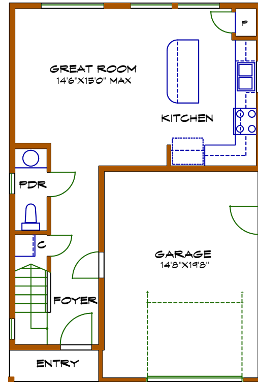
MAIN FLOOR PLAN AREA: 537 SF TOTAL AREA: 993 SF
